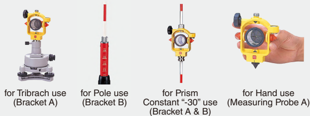
Bracket A
