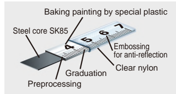
Tape structure
