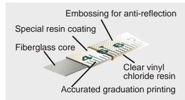
Tape structure
