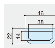
Dimensions 5m / 3sec. (MST-53)
