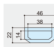
Dimensions 3m / 3sec. (MST-33)
