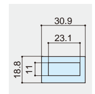
Dimensions (MTR-33)
